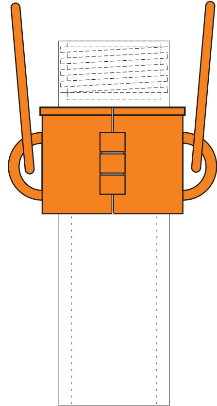
Shur-Grip hybrid well connection to a Johnson Screens' of stainless steel well screen. Shur-Grip casing can also connect to a Johnson Screens brand of PVC well screen.
